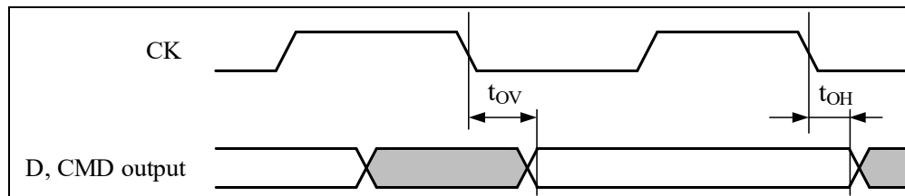
Figure 4-42 SDMMC DDR Mode
