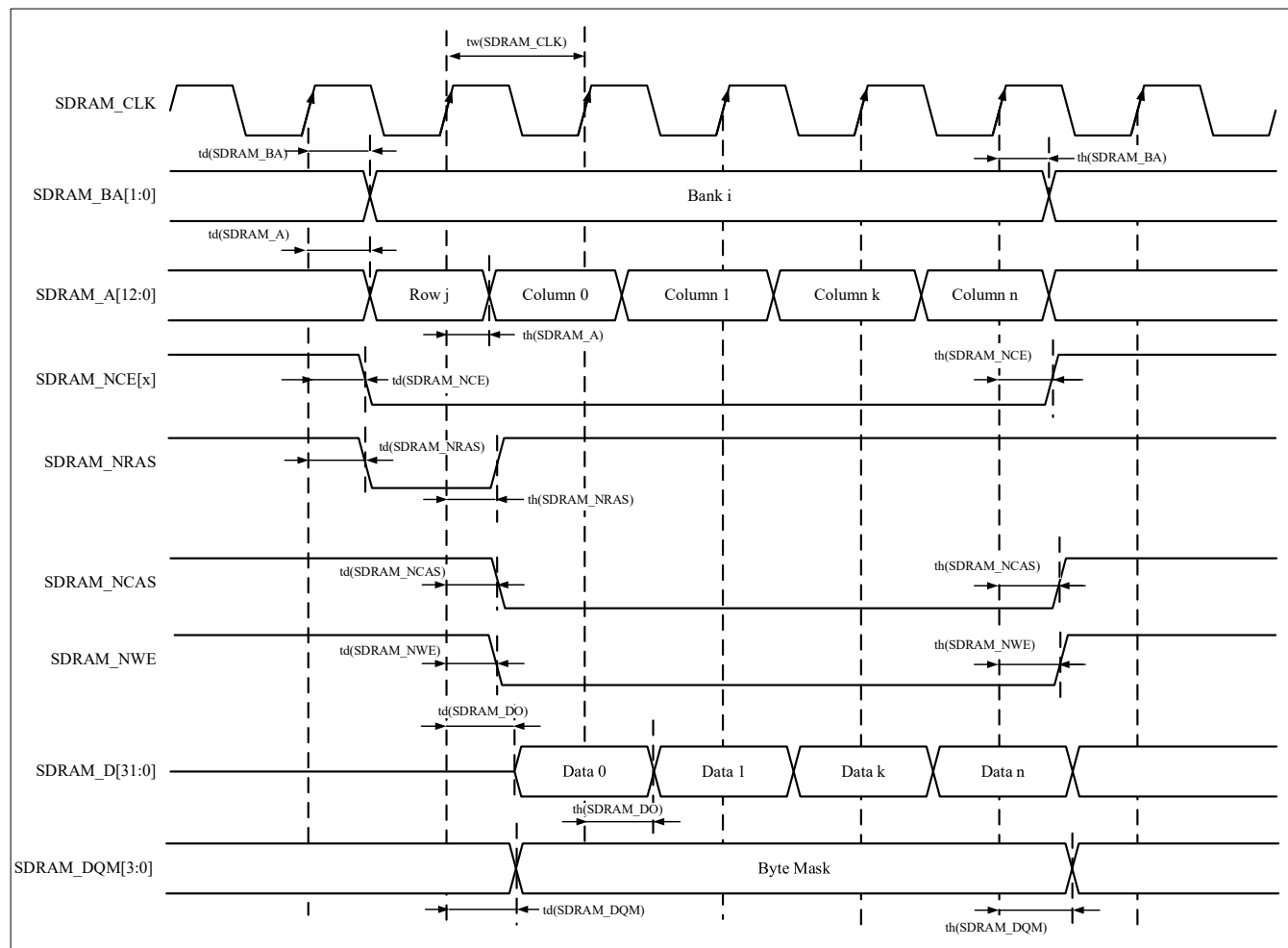
Figure 4-14 SDRAM Write Timing Diagram
