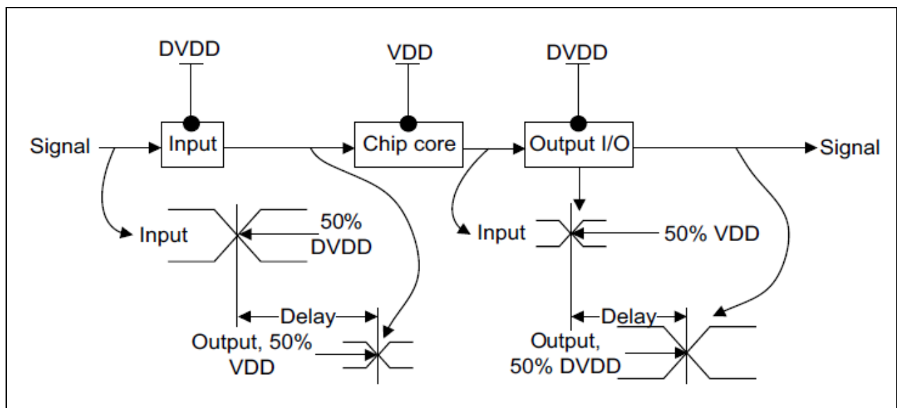
Figure 4-2 Transmission Delay
