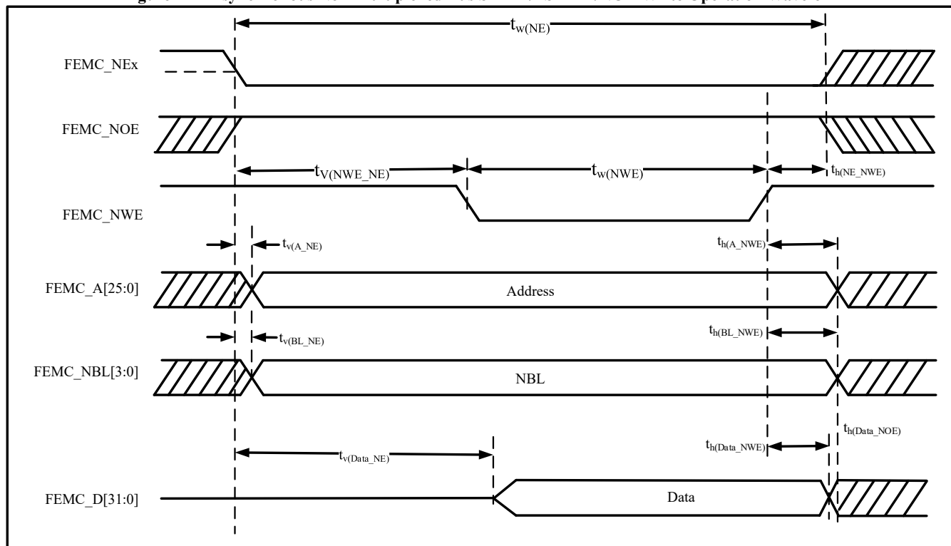
Figure 4-27 Asynchronous Non-Multiplexed Bus SRAM/PSRAM/NOR Write Operation Waveform
