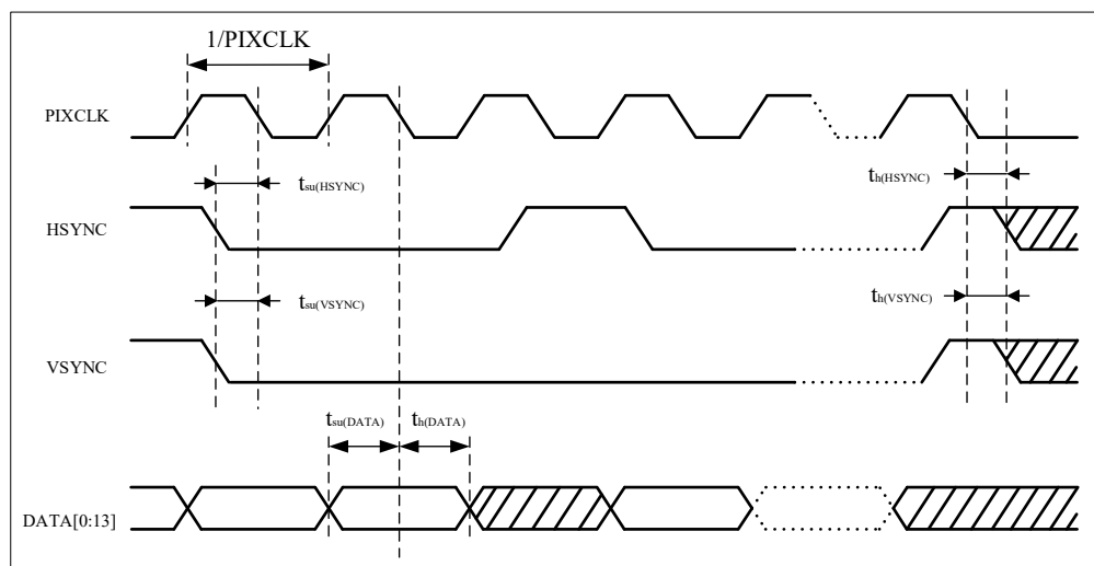
Figure 4-47 DVP Interface Timing Diagram
