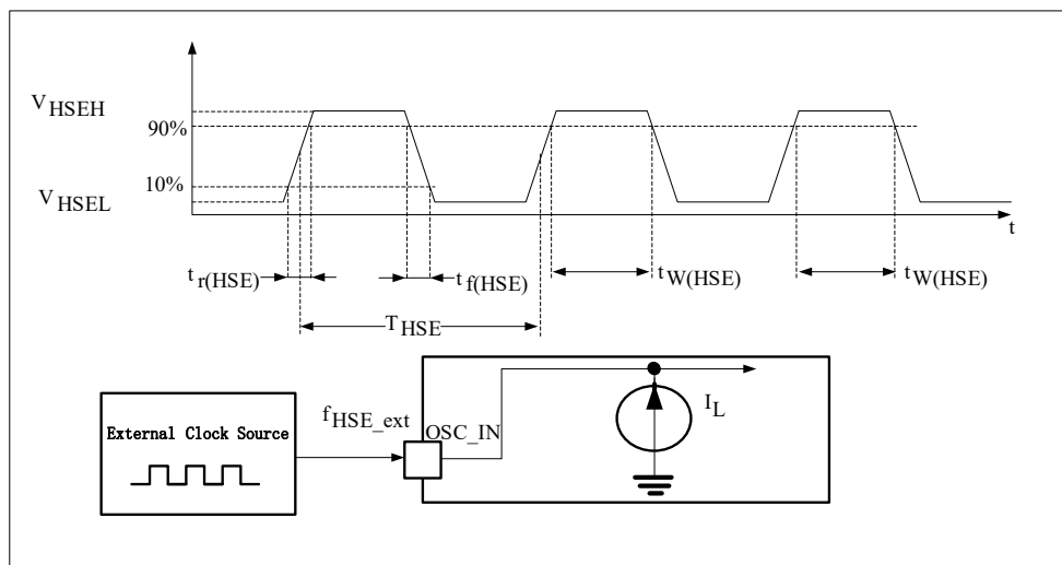
Figure 4-6 AC timing diagram for external high-speed clock source
