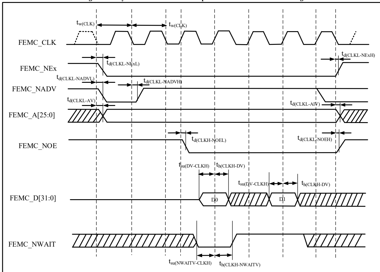
Figure 4-30 Synchronous Non-Bus-Multiplexed NOR/PSRAM Read Timing
