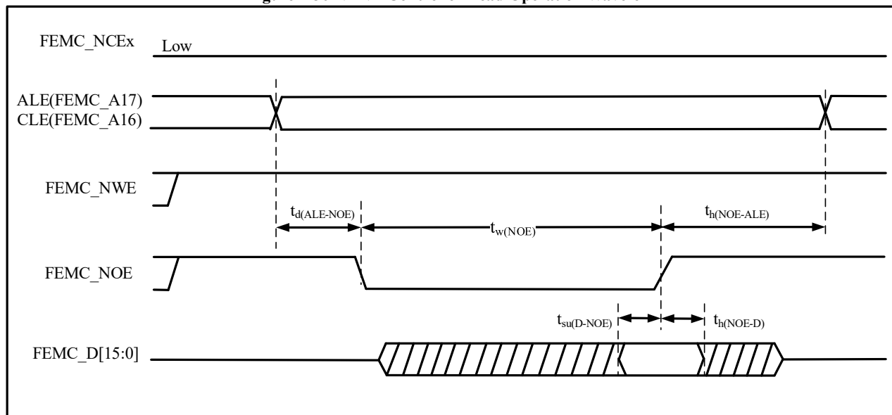
Figure 4-36 NAND Controller Read Operation Waveform
