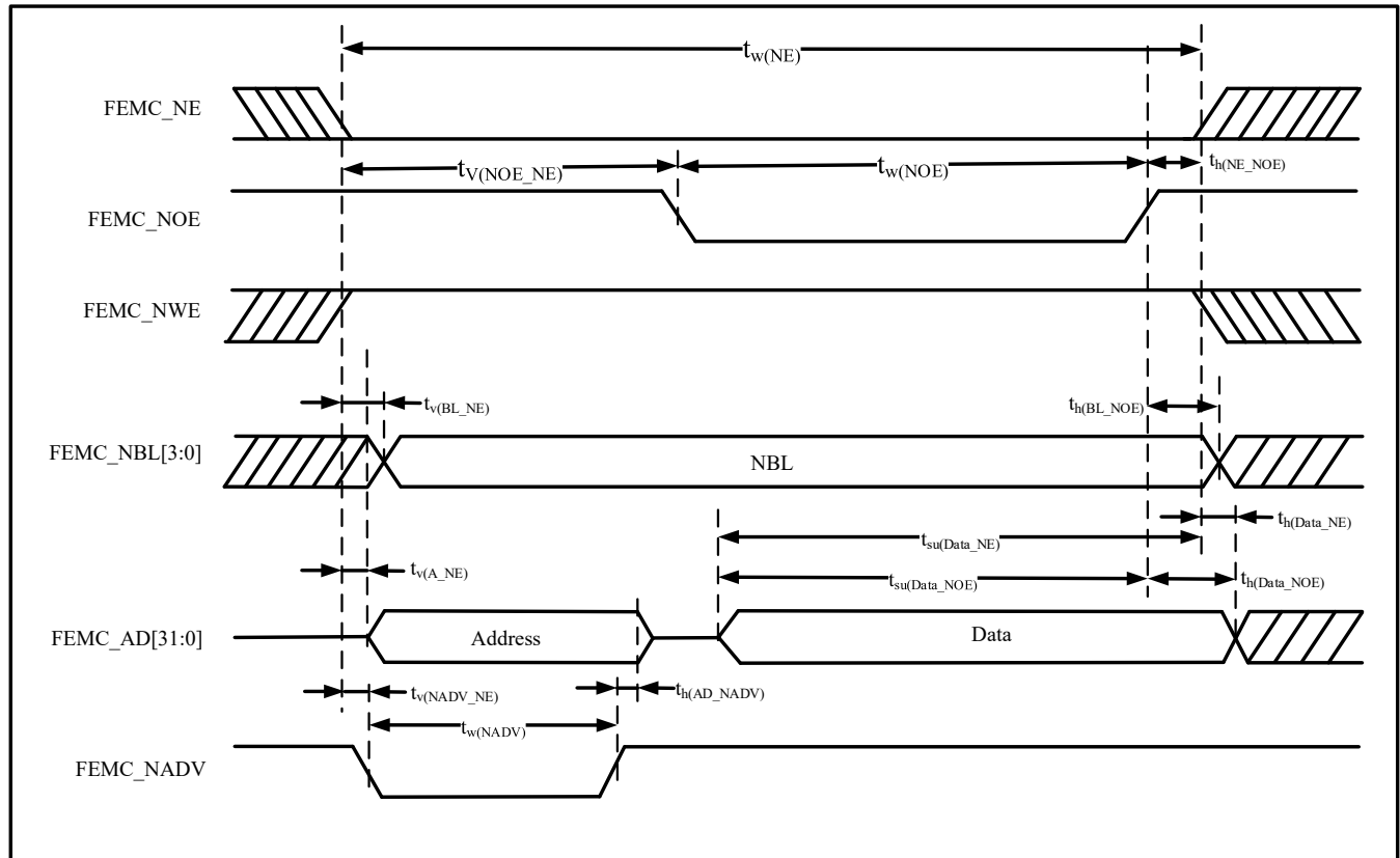
Figure 4-28 Asynchronous Bus Multiplexed PSRAM/NOR Read Operation Waveform
