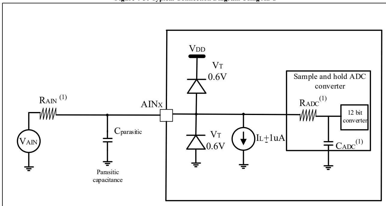
Figure 4-50 Typical Connection Diagram Using ADC
