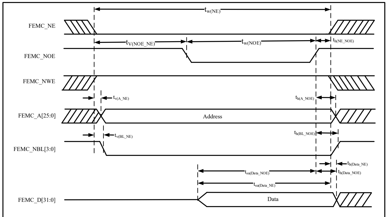
Figure 4-26 Asynchronous Non-Multiplexed Bus SRAM/PSRAM/NOR Read Operation Waveform
