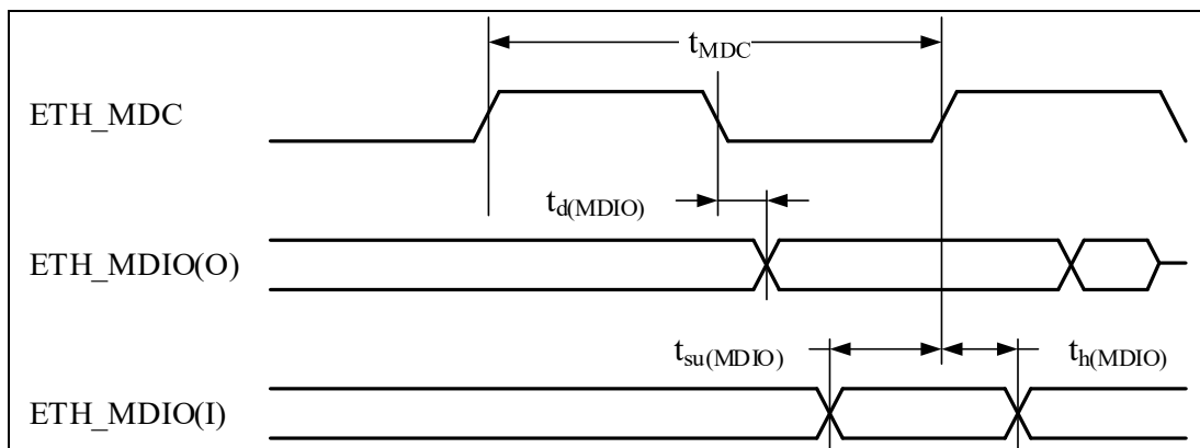
Figure 4-43 MDIO/SMA Timing Diagram
