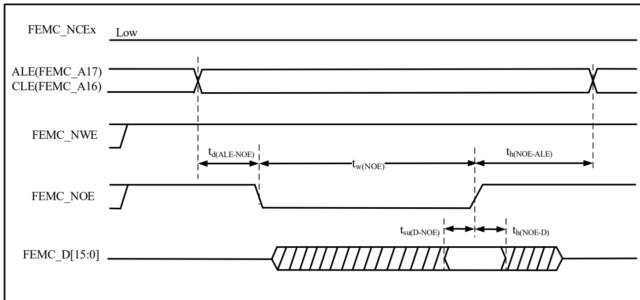
Figure 4-34 NAND Controller Read Operation Waveform
