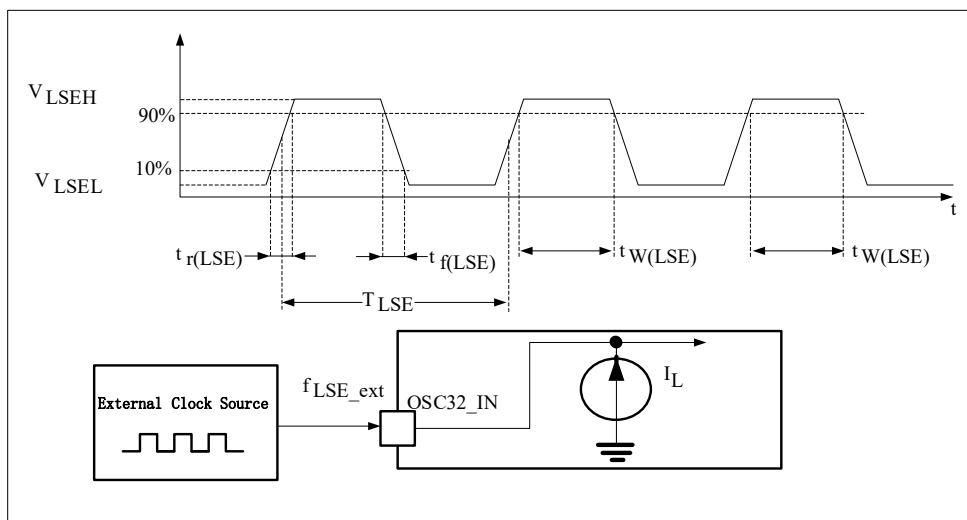
Figure 4-7 AC timing diagram for external low-speed clock source
