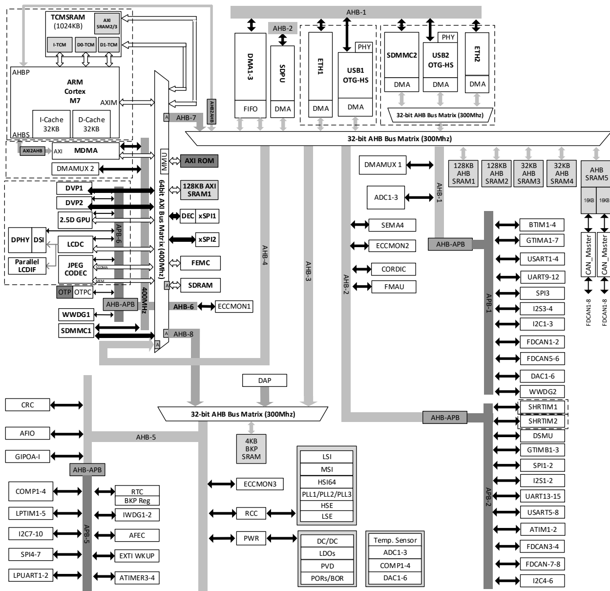
Figure 1-1 N32H760System Block Diagram
