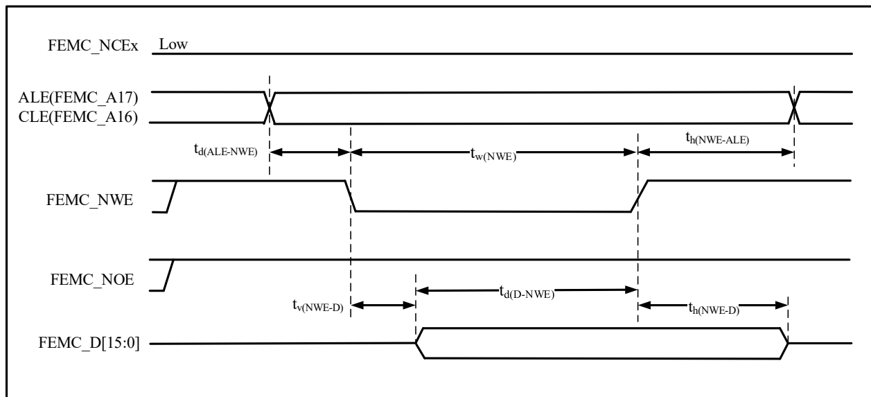
Figure 4-39 NAND Controller Write Operation Waveform
