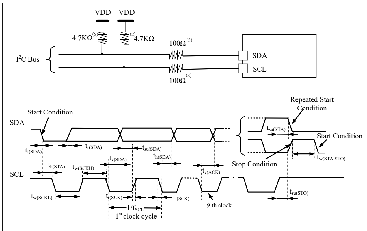
Figure 4-15: I2C Bus AC Waveform and Measurement Circuit (1)
