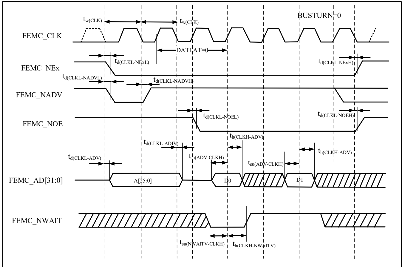
Figure 4-32 Synchronous Bus-Multiplexed NOR/PSRAM Read Timing
