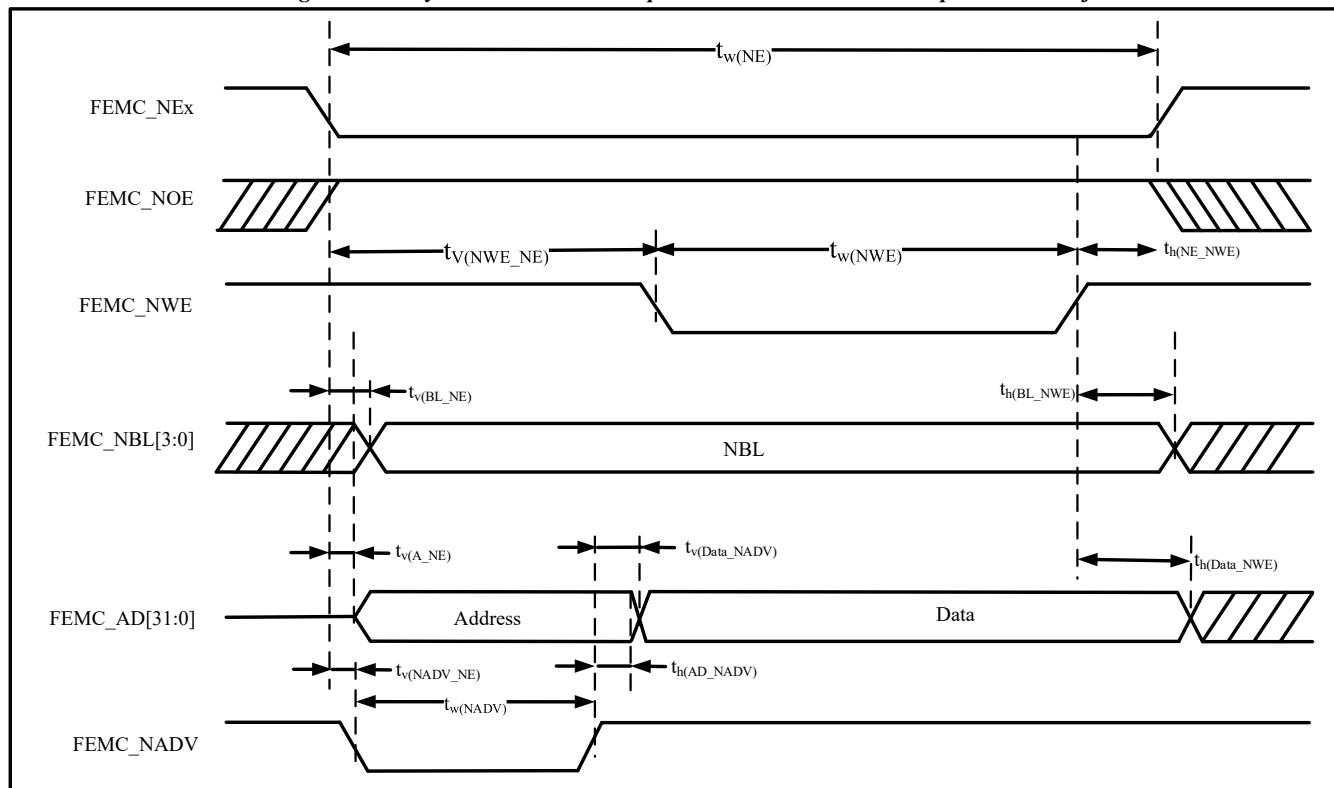
Figure 4-29 Asynchronous Bus Multiplexed PSRAM/NOR Write Operation Waveform
