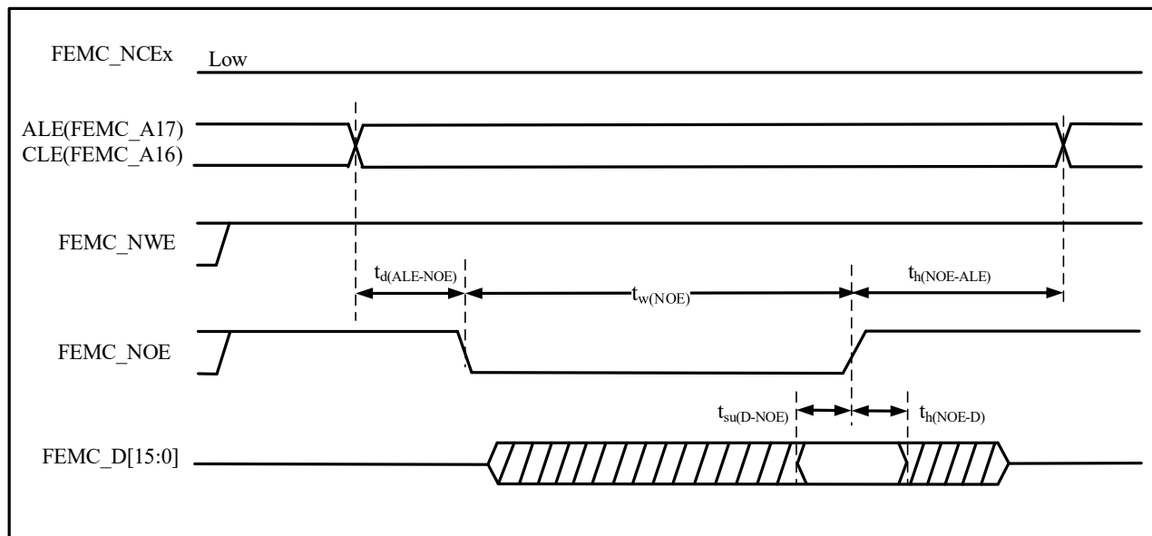
Figure 4-38 NAND Controller Read Operation Waveform
