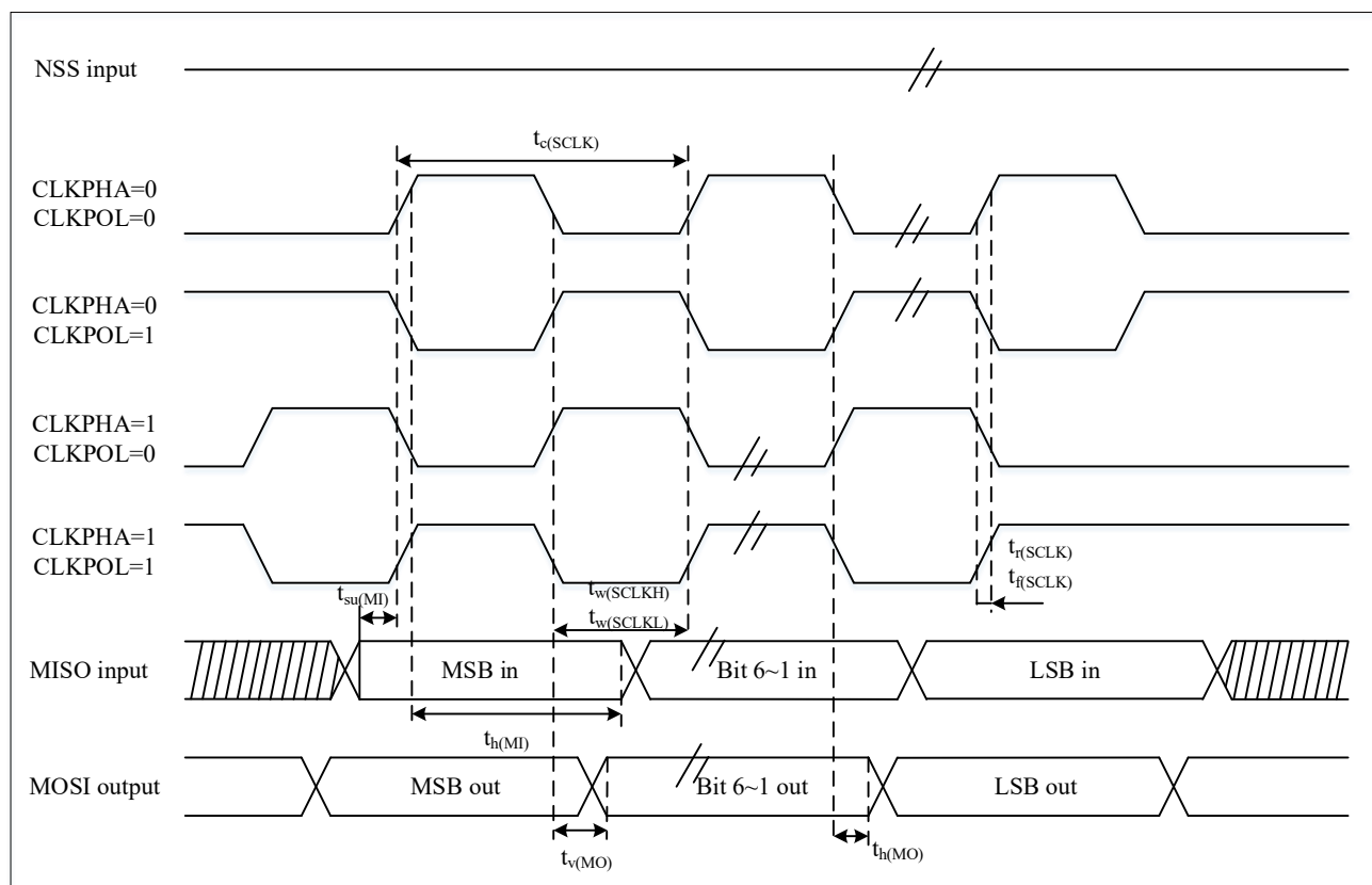
Figure 4-18 SPI Timing Diagram — Master Mode (1)
