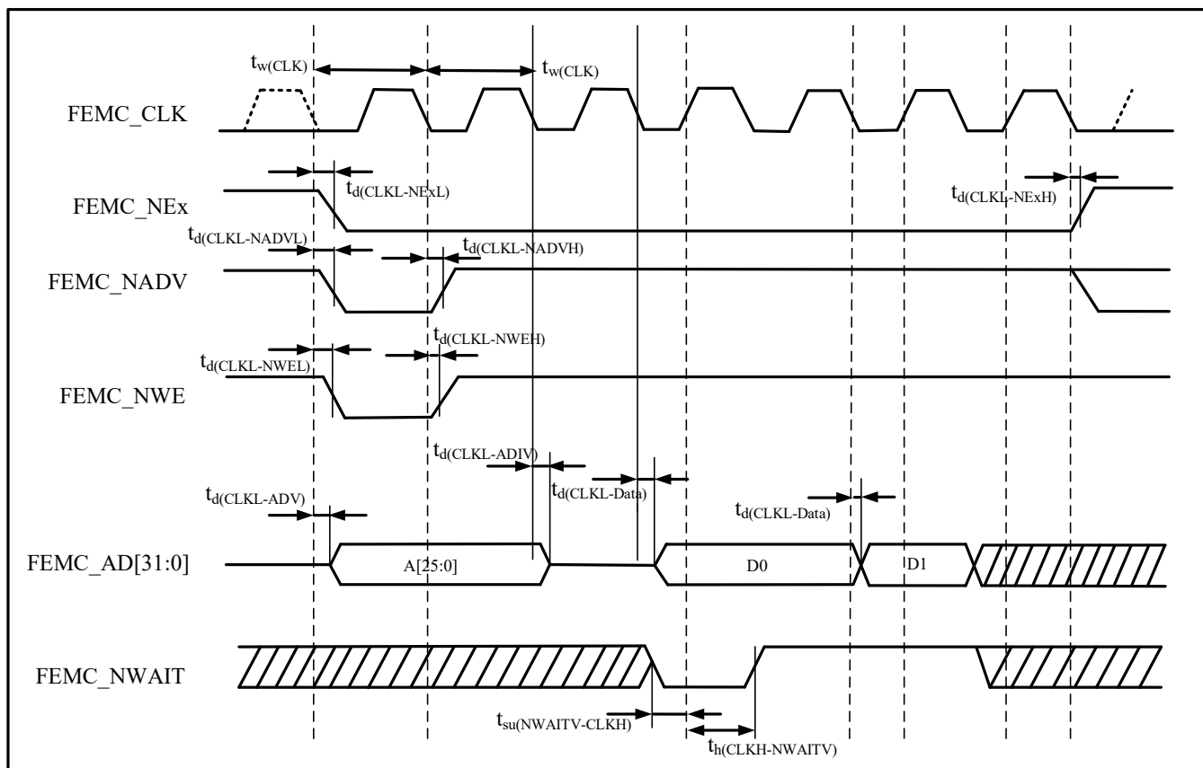
Figure 4-33 Synchronous Bus-Multiplexed PSRAM Write Timing
