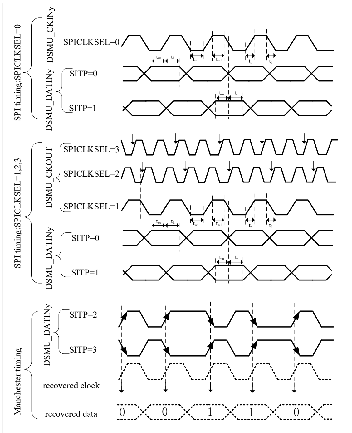
Figure 4-48 DSMU Channel Transceiver Timing Diagram
