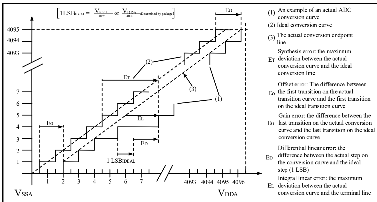
Figure 4-49 ADC Accuracy Characteristics
