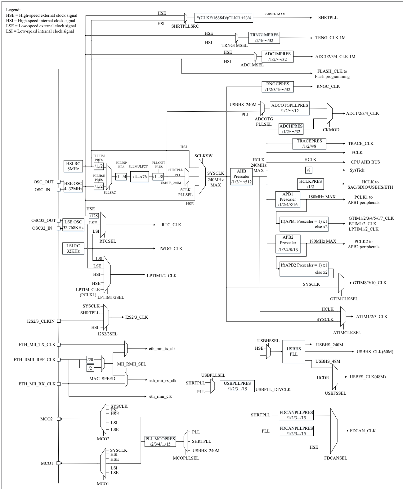
Figure 2-2 Clock Tree
