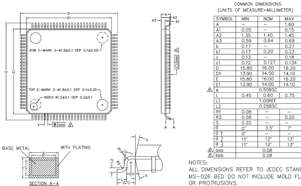
Figure 5-3 LQFP100 Package Dimensions
