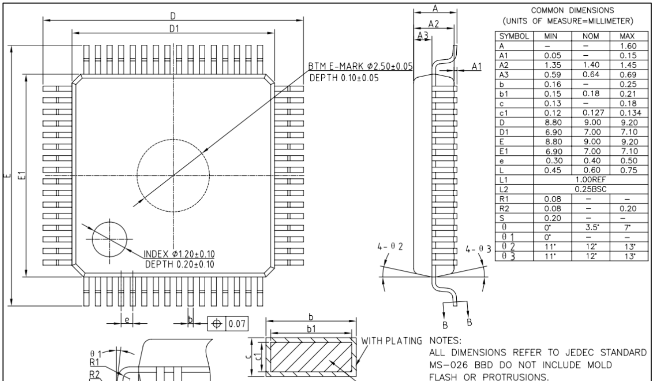
Figure 5-5 LQFP64(7mm×7mm) Package Dimensions
