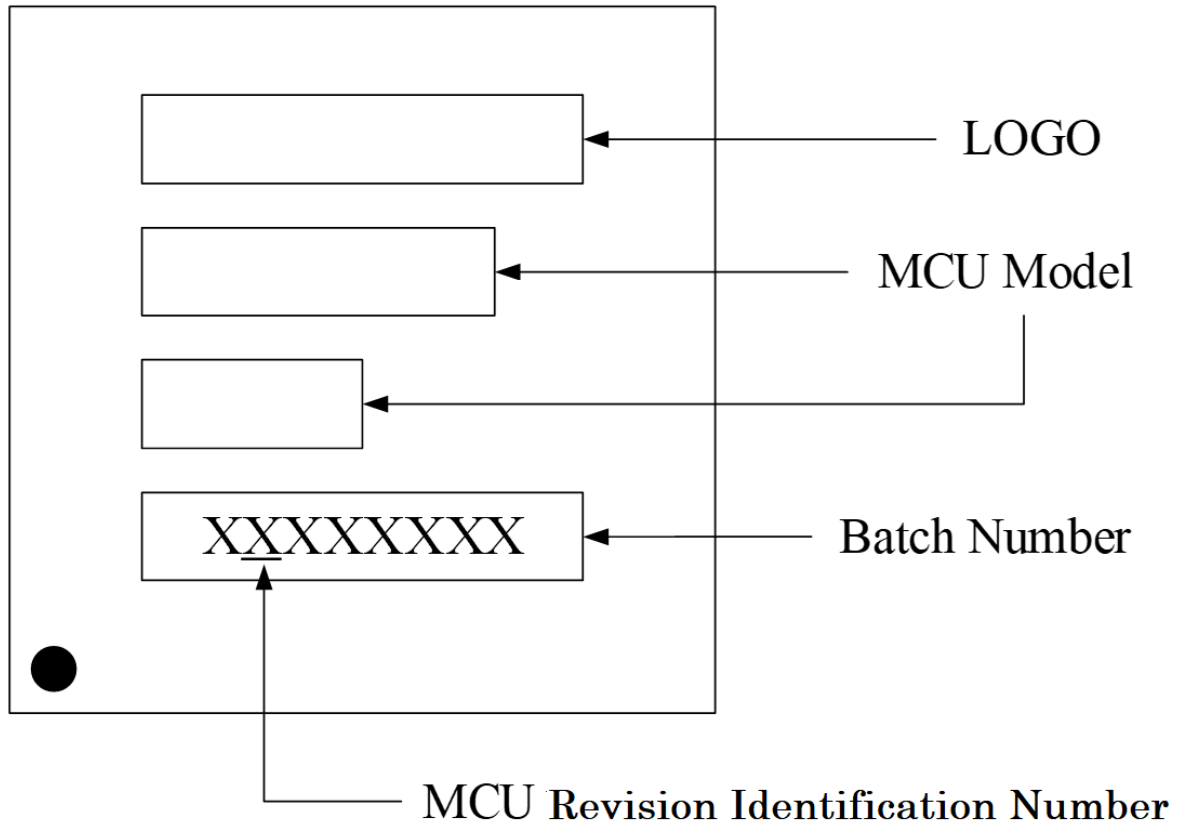
Figure 5-6 Marking Information
