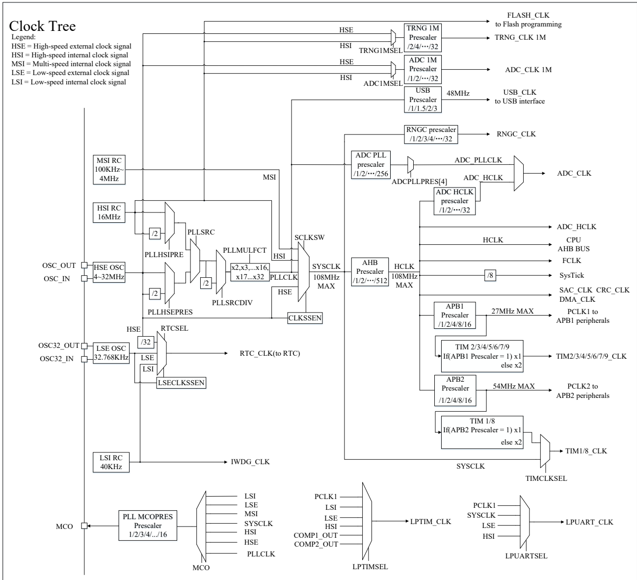
Figure 2-2 Clock Tree
