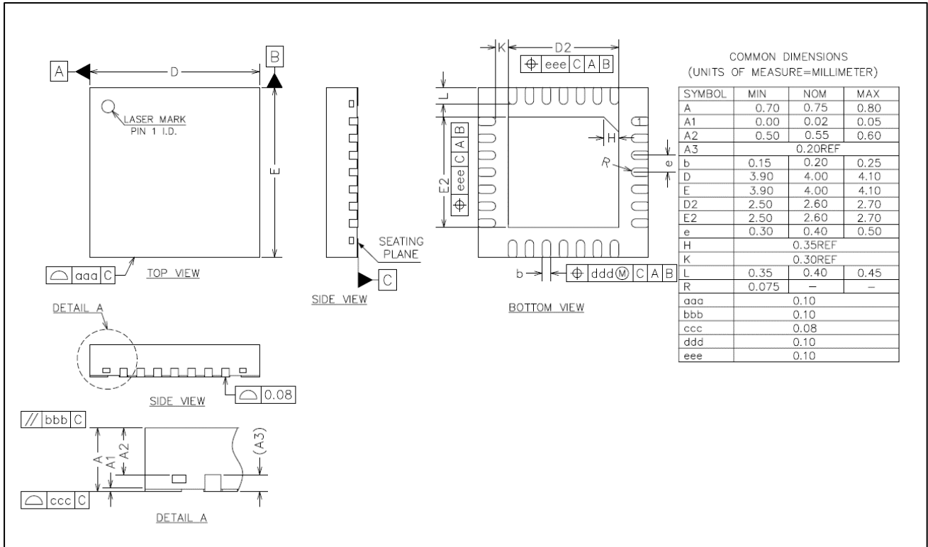
Figure 5-1 QFN28(4mmx4mm) Package Dimensions
