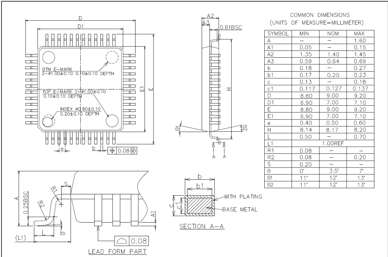
Figure 5-3 LQFP48(7mmx7mm) Package Dimensions
