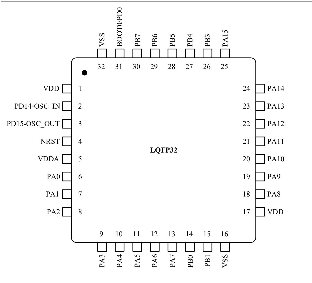
Figure 3-2 N32G435 Series LQFP32 Pinout
