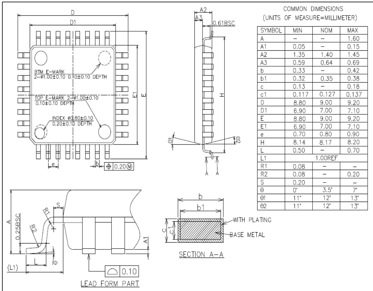
Figure 5-2 LQFP32(7mmx7mm) Package Dimensions
