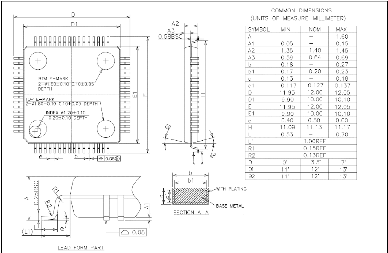
Figure 5-4 LQFP64 (10mm×10mm) Package Dimensions
