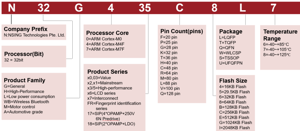
Figure 1-2 N32G435 C 8 L 7
