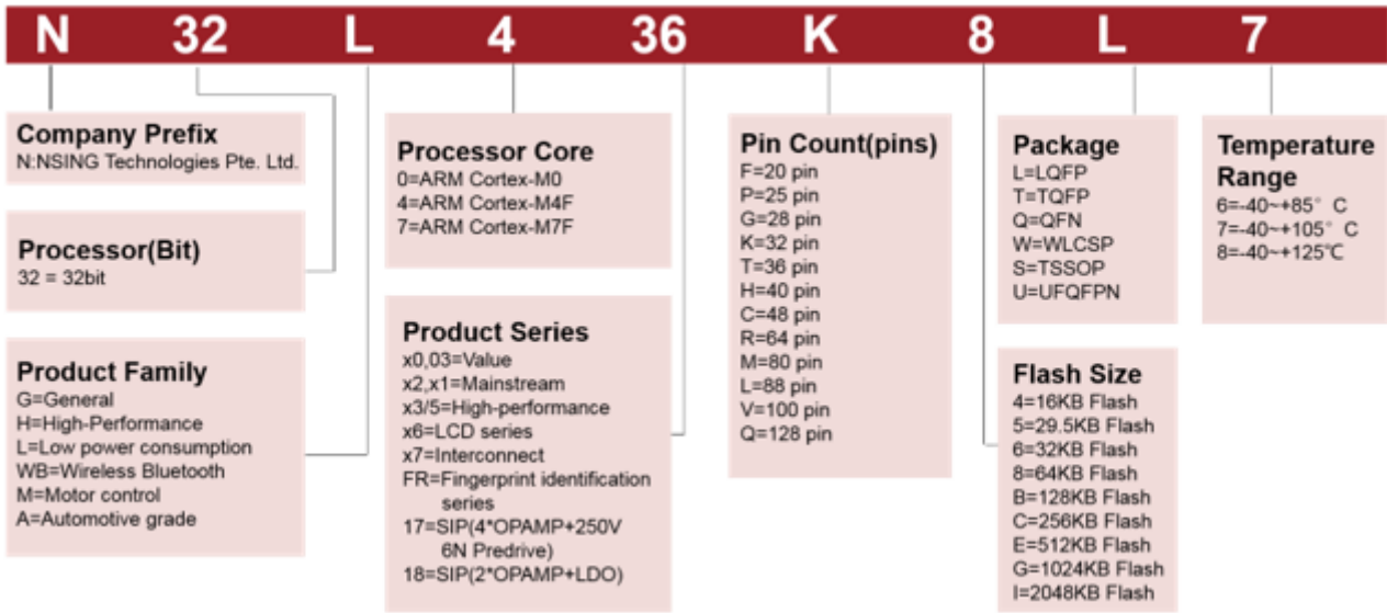
Figure 1-2 N32L436K8L7 Series Part Number Information
