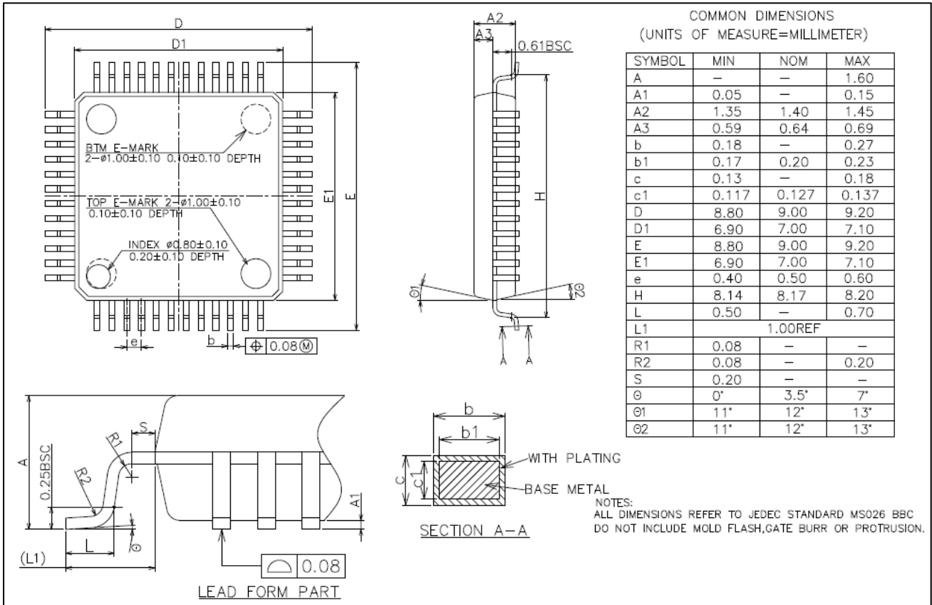
Figure 5-2 LQFP48(7mmx7mm) Package Dimensions
