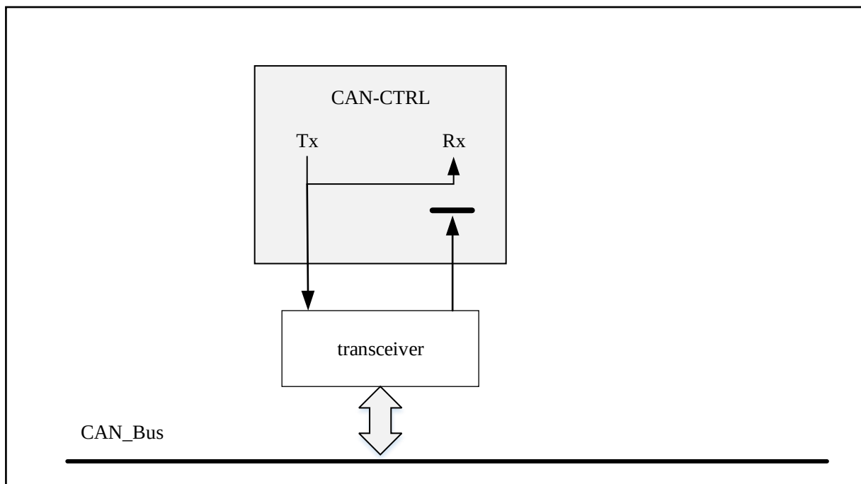
Figure 19-4 loopback mode
