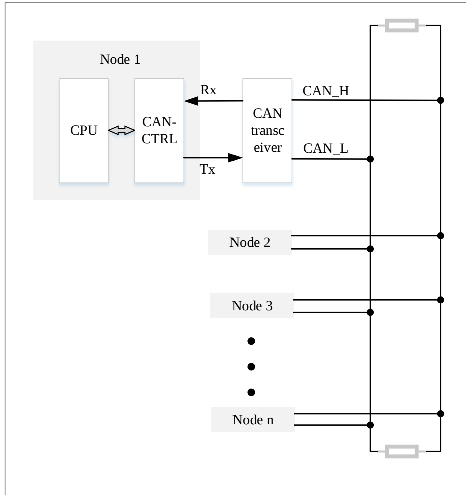
Figure 19-1 Topology of CAN network
