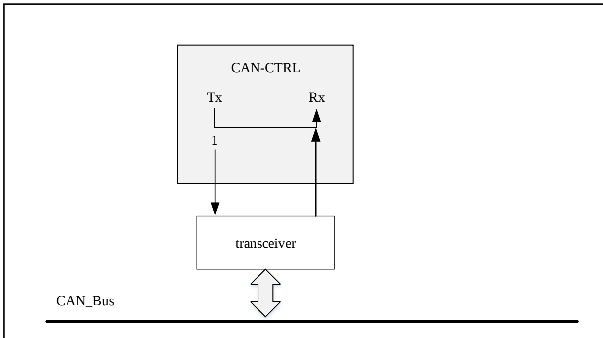
Figure 19-5 silent mode
