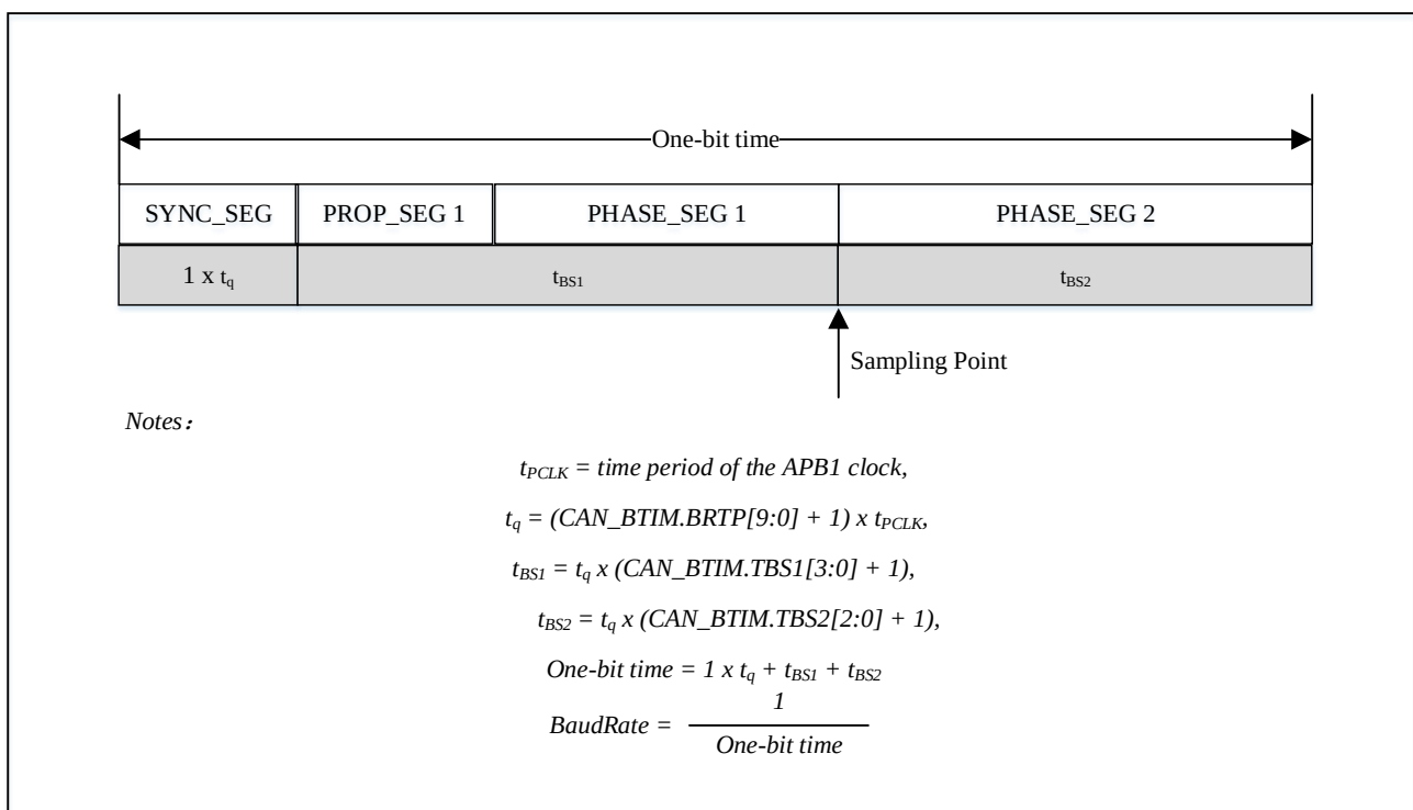
Figure 19-11 Bit sequence
