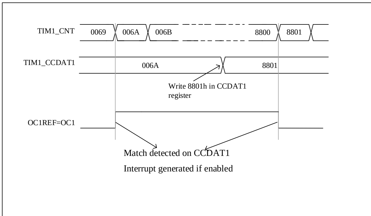
Figure 11-21 Output compare mode, toggle on OC1
