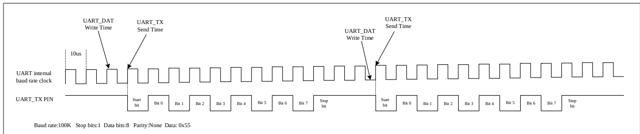
Figure 22-5 Transmission time difference
