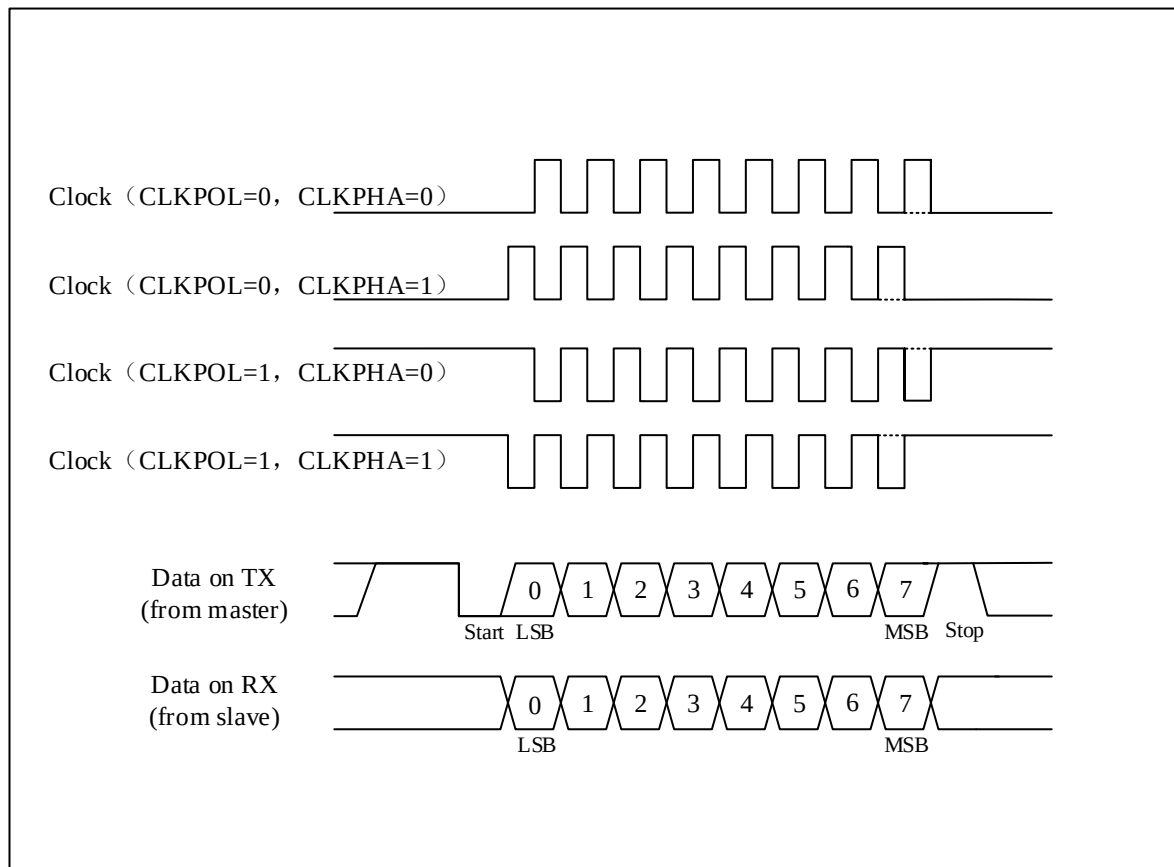
Figure 22-16 USART data clock timing example (WL=0)
