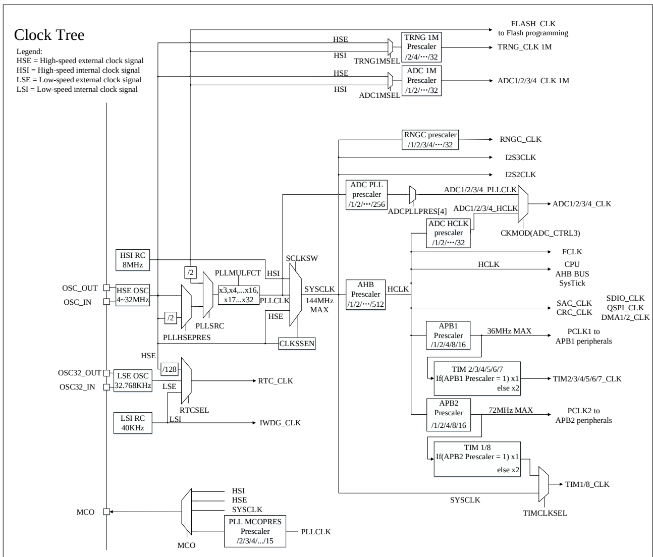
Figure 6-2 Clock Tree
