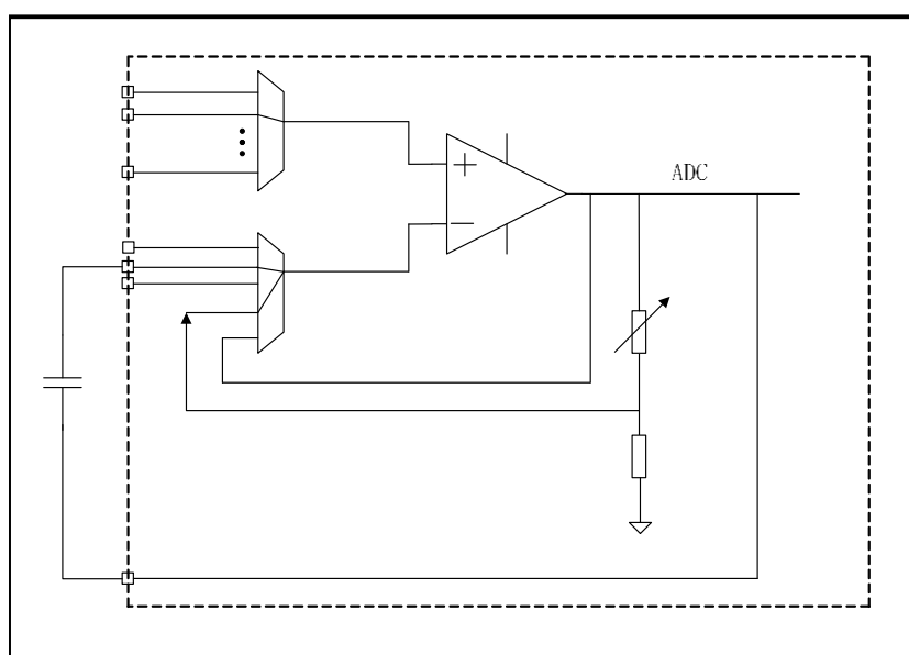
Figure 25-8 Internal gain mode with filter
