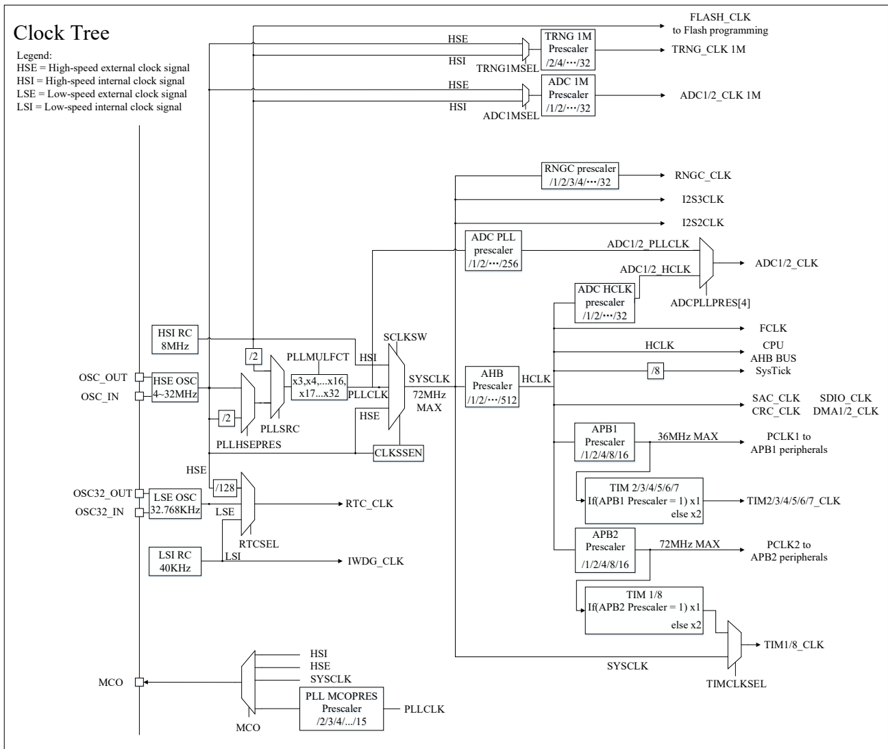
Figure 2-2 Clock tree
