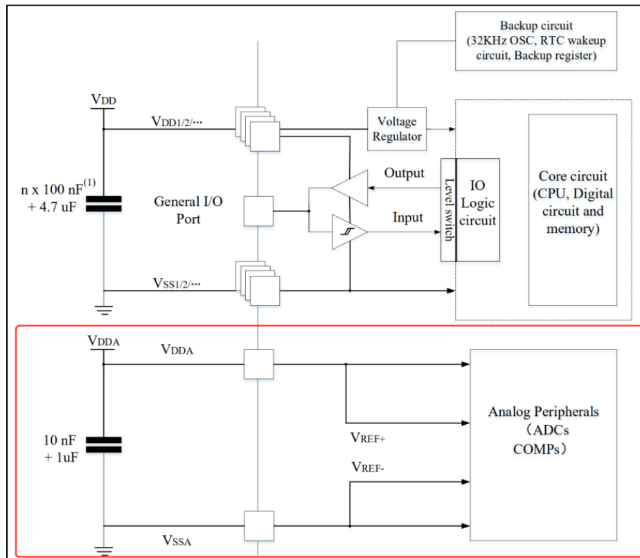
Figure 2-6 Power System
