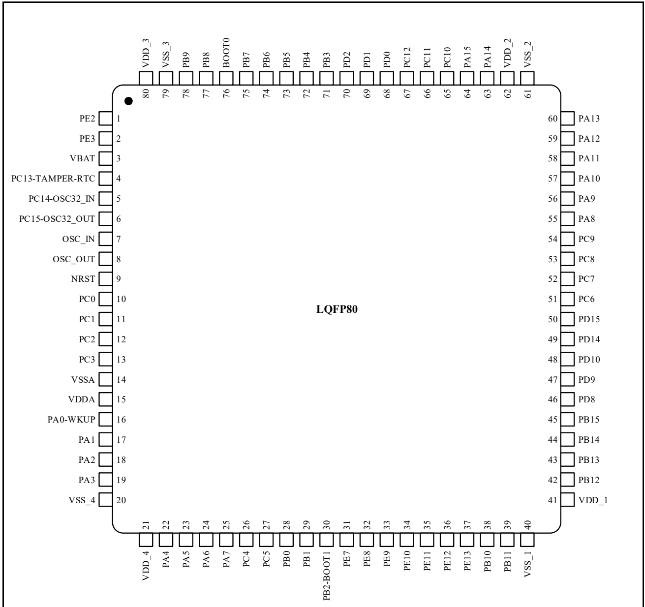
Figure 3-3 N32G452 Series LQFP80 Pinout
