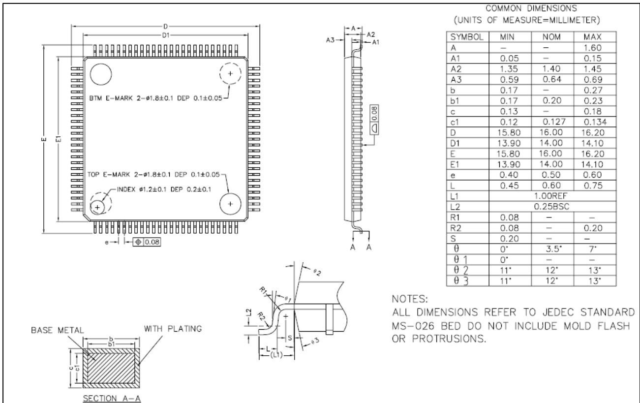
Figure 5-4 LQFP100 Package Dimensions
