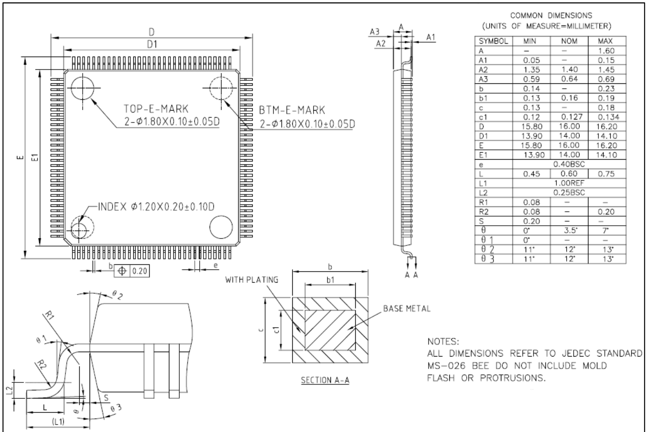
Figure 5-5 LQFP128 Package Dimensions
