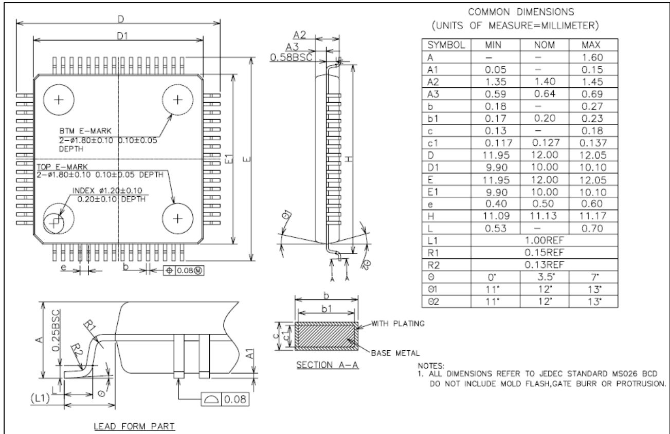
Figure 5-3 LQFP80 Package Dimensions
