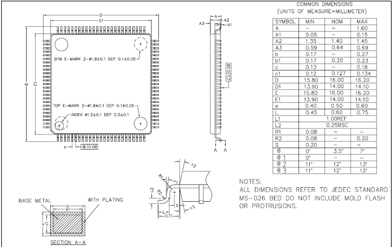
Figure 5-6 LQFP100 package dimensions
