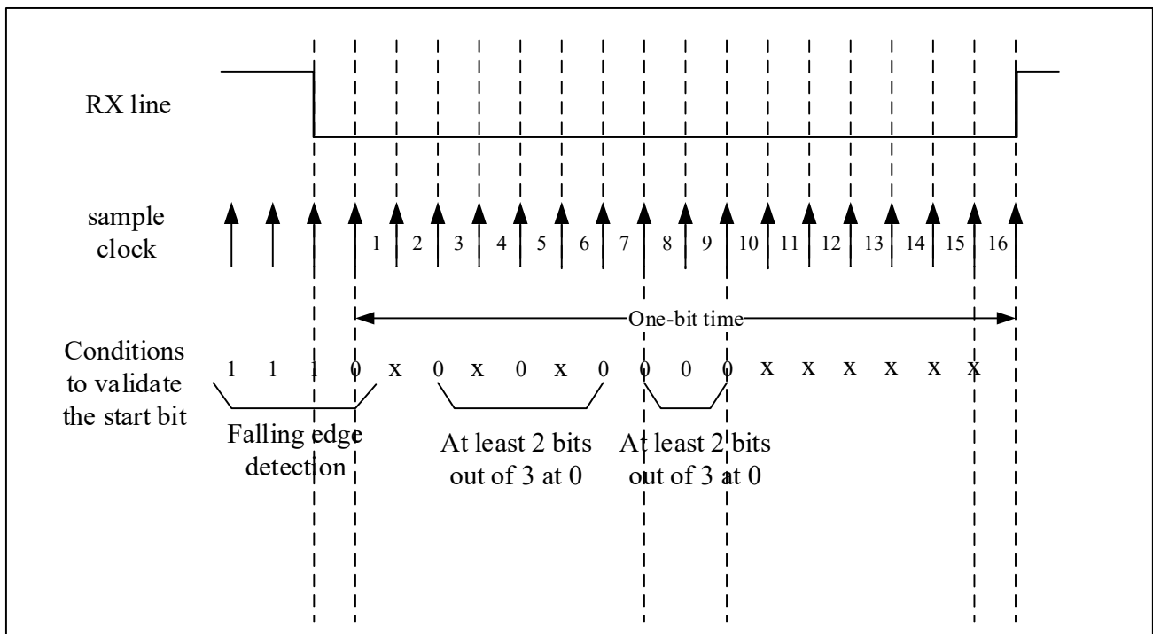
Figure 18-6 Start Bit Detection
