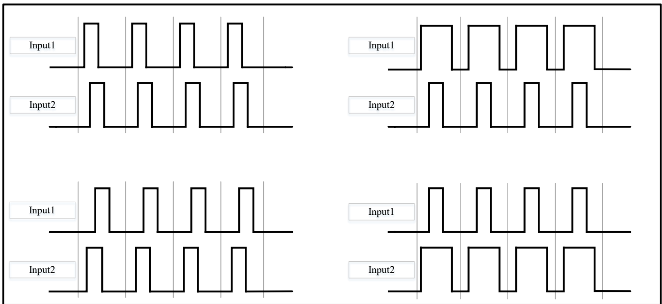
Figure 12-9 Input1 and Input2 Input Waveforms When Decoder Module Is Not Operating
