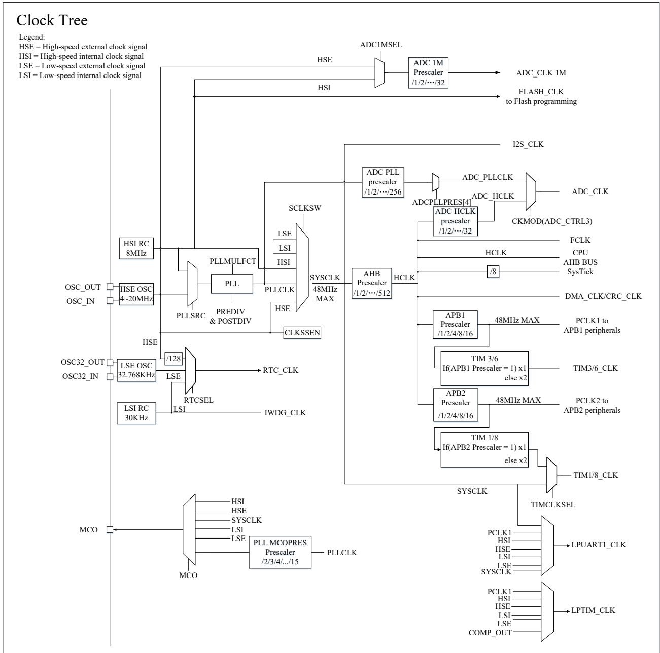
Figure 4-2 Clock Tree
