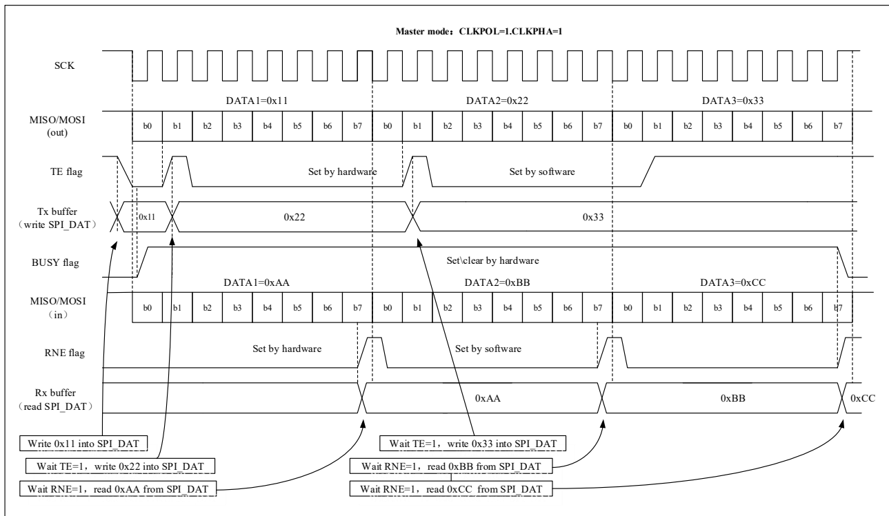
Figure 20-5 Changes of TE/RNE/BUSY During Continuous Transmission in Master Full Duplex Mode
