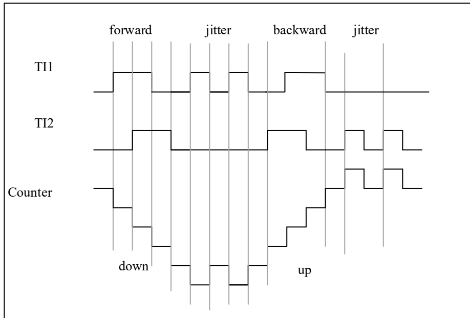
Figure 10-28 Encoder Interface Mode Example with IC1FP1 Polarity Inverted
