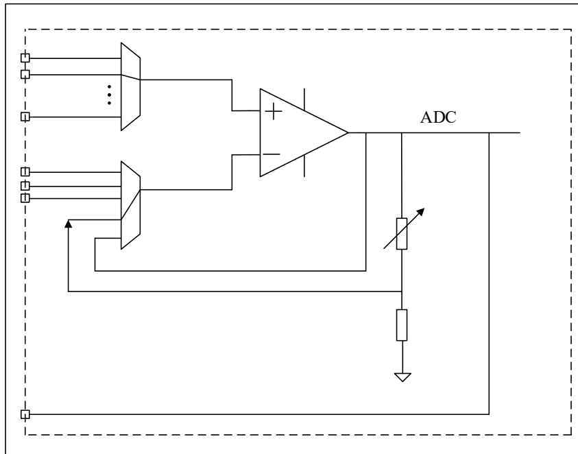
Figure 22-4 OPAMP Programmable Gain Mode
