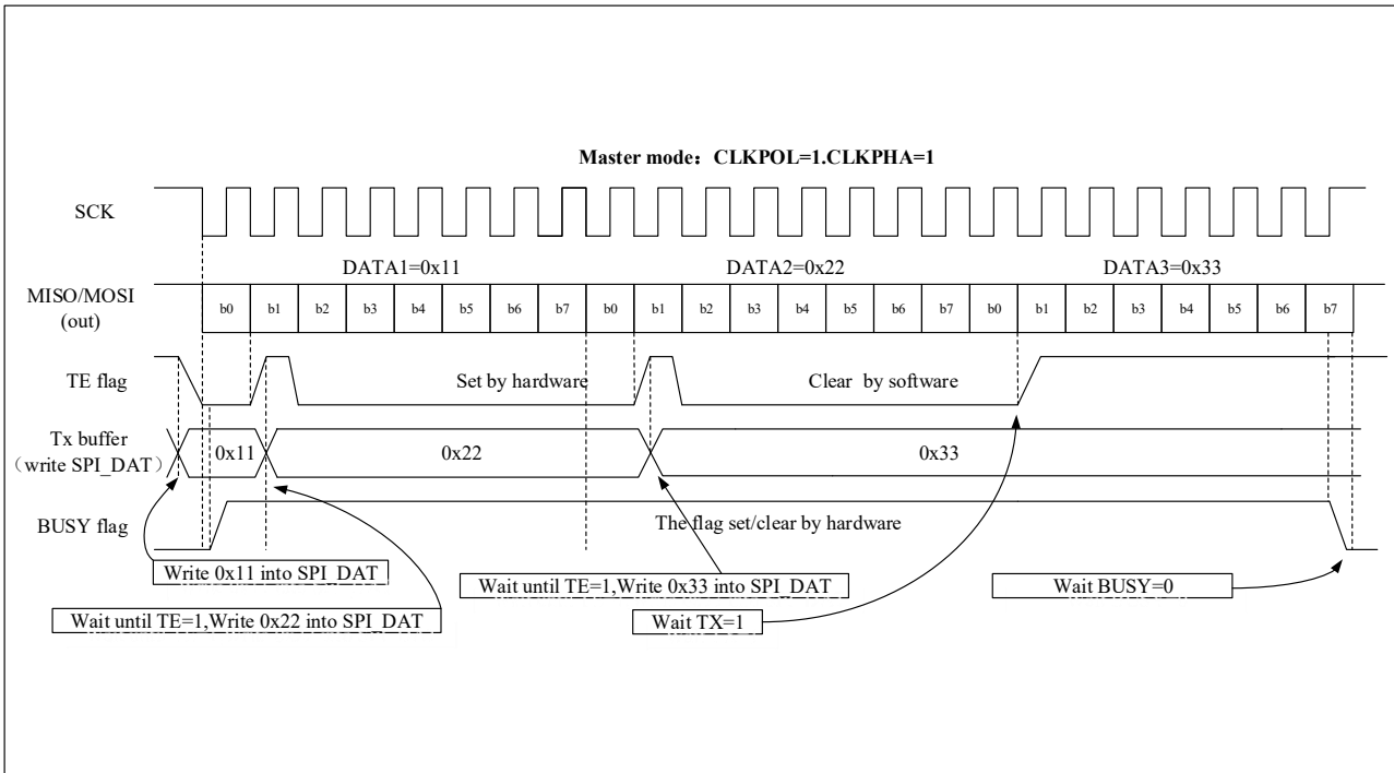
Figure 20-6 Changes of TE/BUSY During The Host Transmits Continuously in One-way Transmit-only Mode
