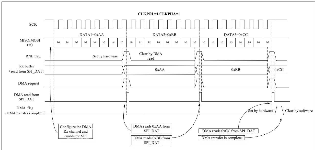
Figure 20-12 Reception Using DMA
